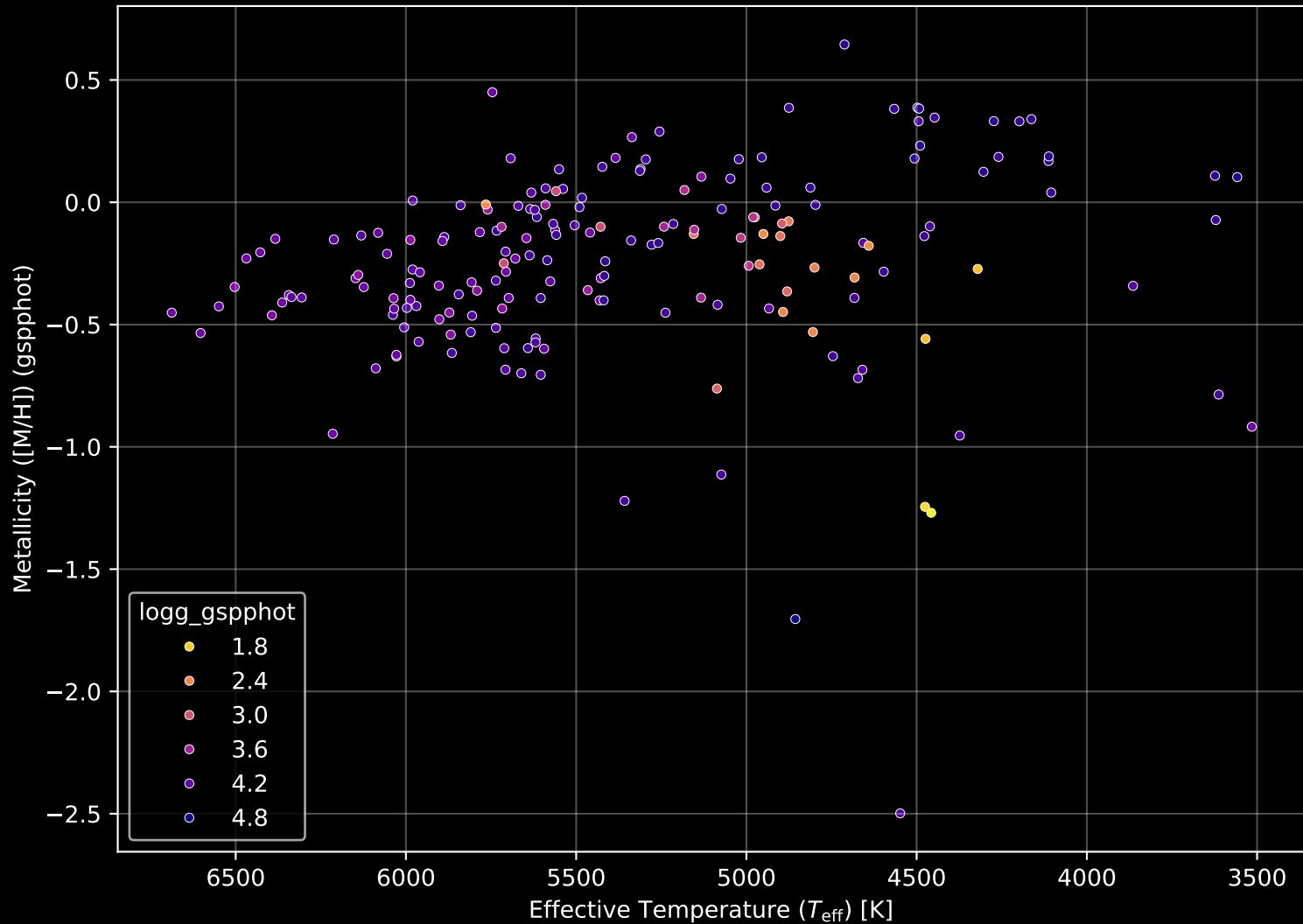
APOGEE DR17 Field: [134+66_MGA] Stellar Population Parameters (n= 185)
