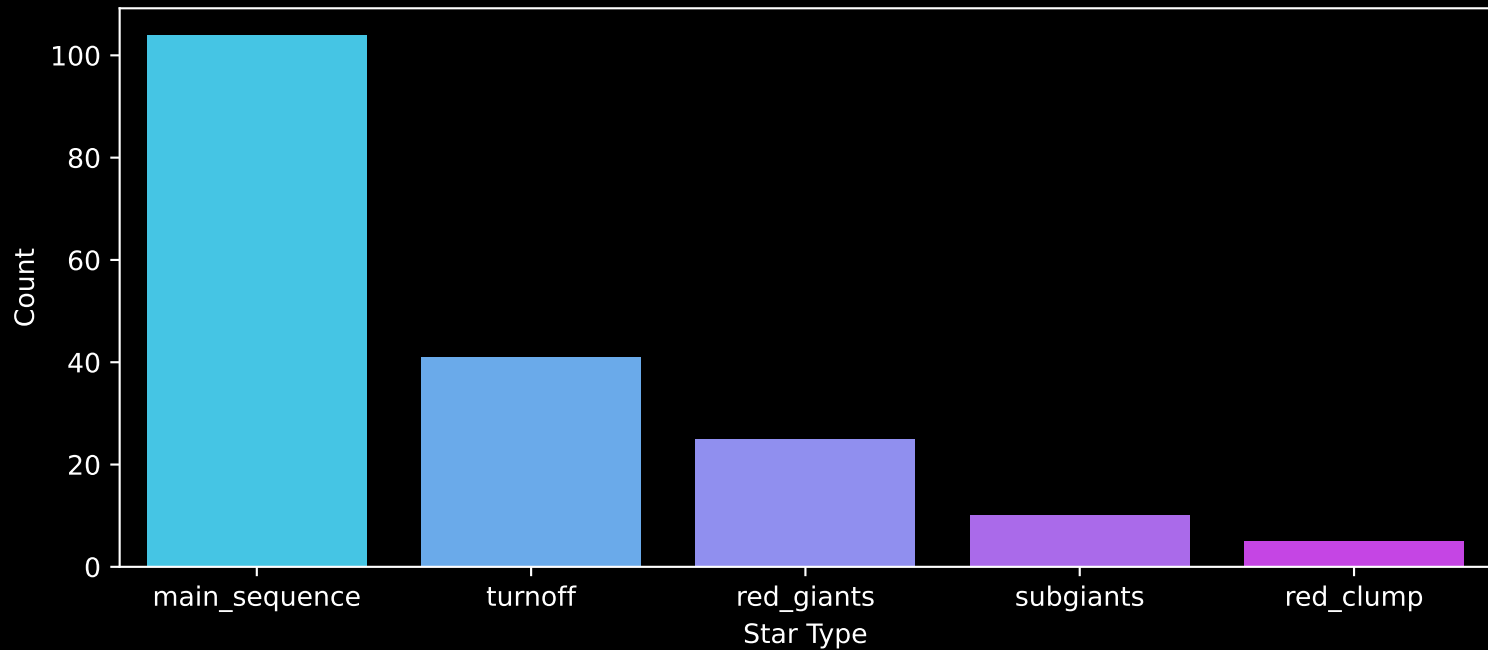
APOGEE DR17 Field: [134+66_MGA] Count plot of Star Type
