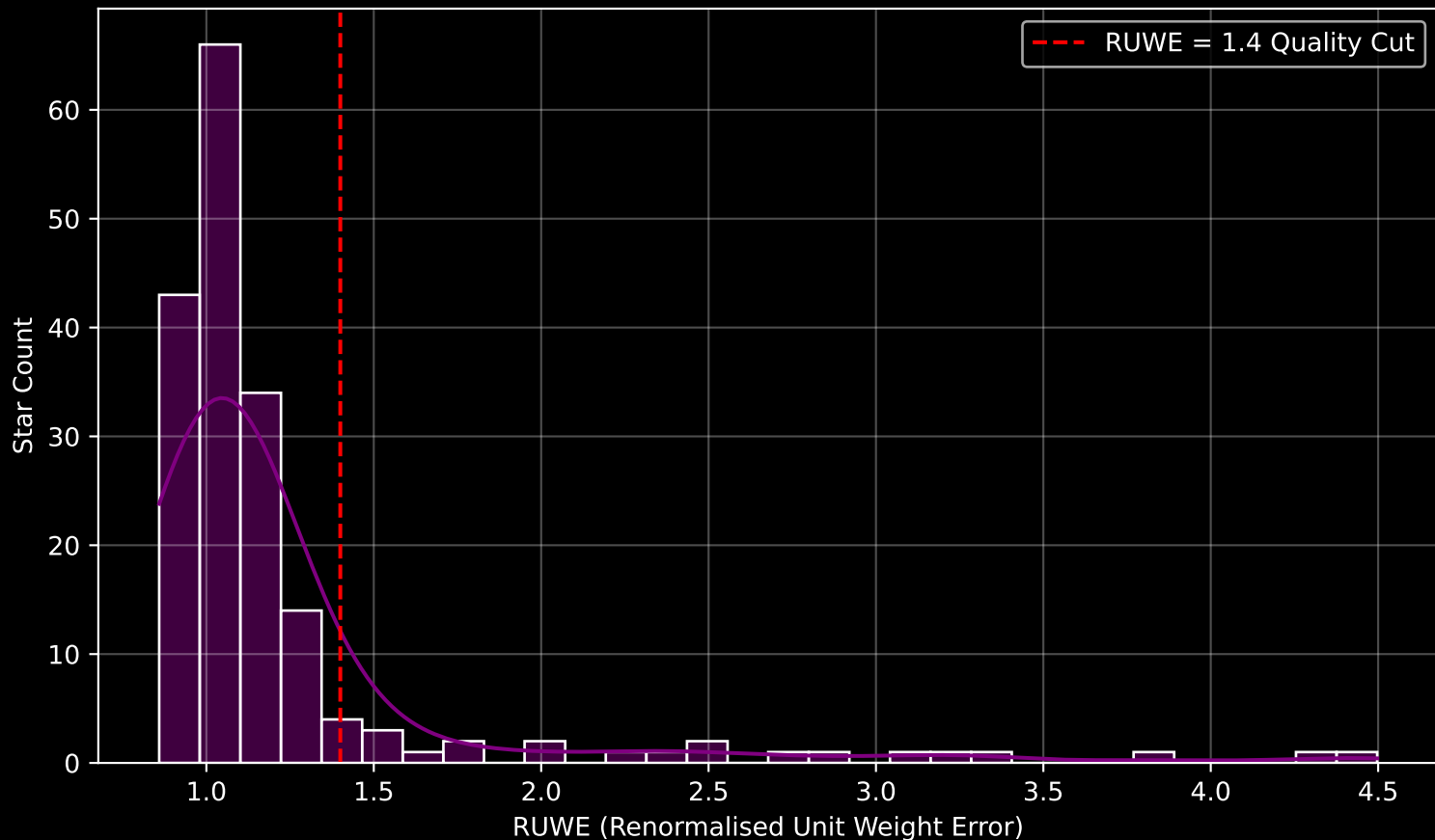
GAPOGEE DR17 Field [134+66_MGA] RUWE Distribution (n= 181)
