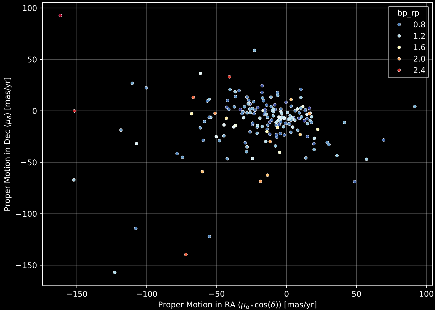
APOGEE DR17 Field: [134+66_MGA] Proper Motion Diagram (n= 185)
