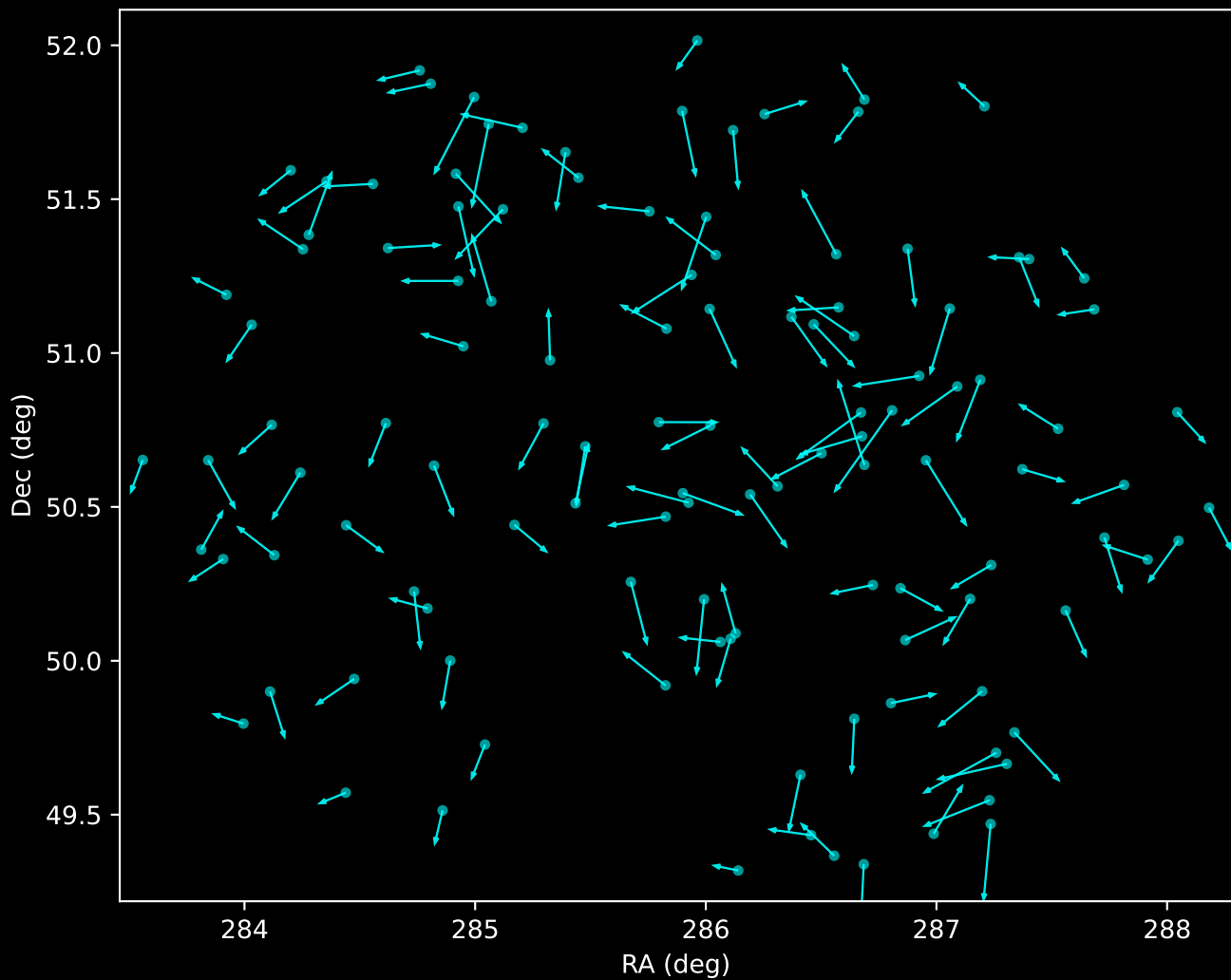
APOGEE DR17 Noise Stream Proper Motion Vectors (n=119)
