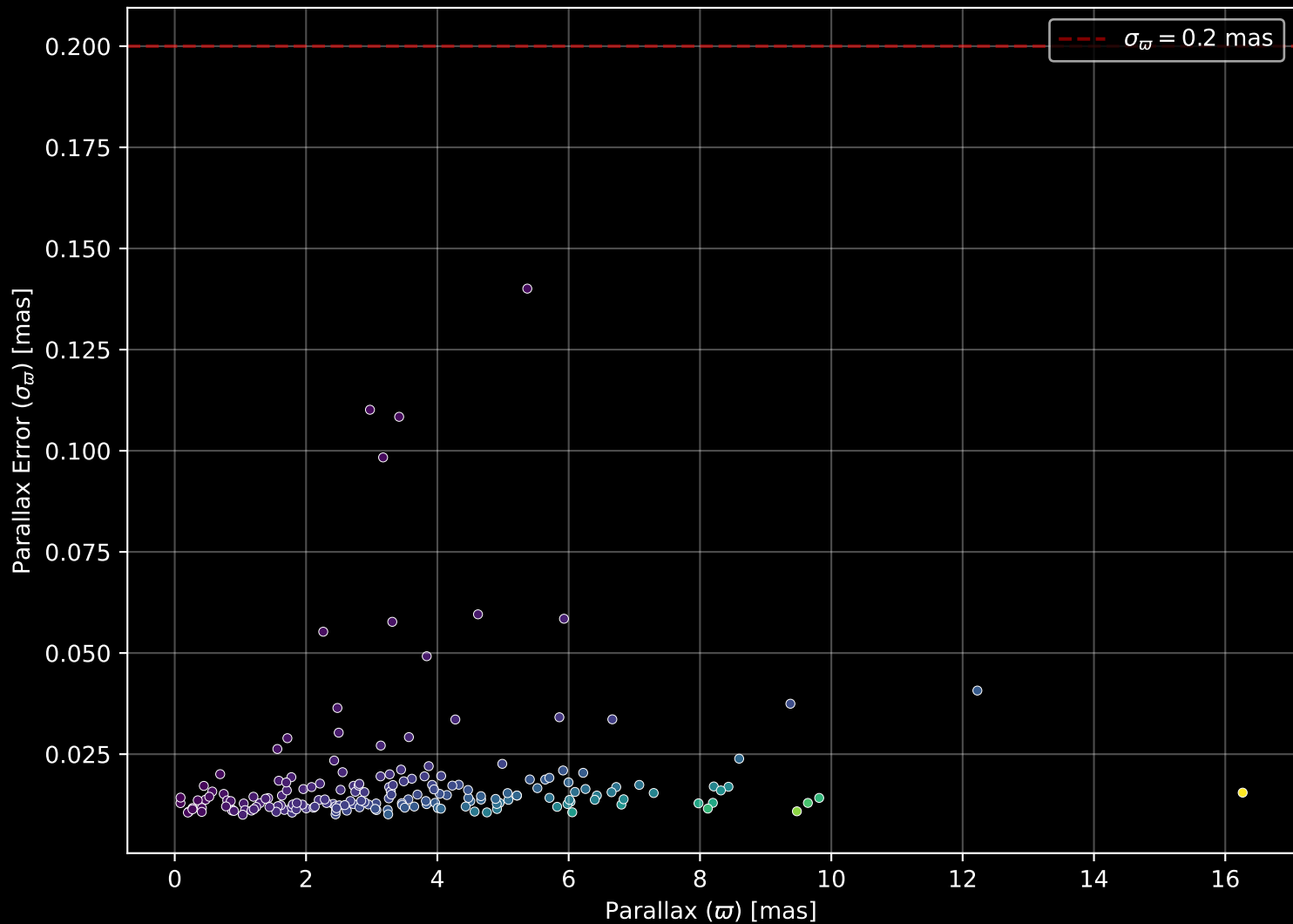
APOGEE DR17 Field: [134+66_MGA] Parallax Quality (n= 185)
