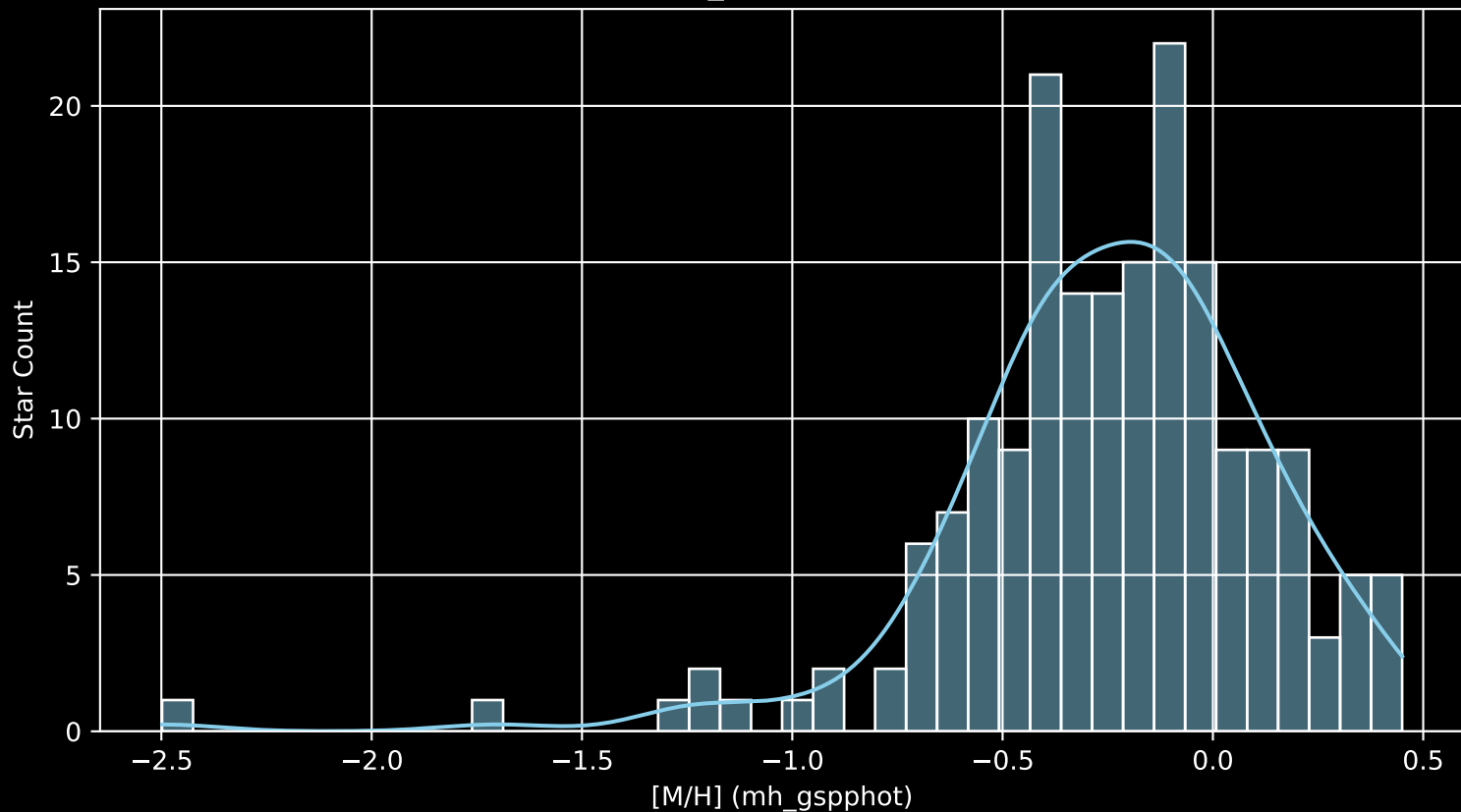
APOGEE DR17 Field: [134+66_MGA [M/H] (mh_gspphot) (n= 184)
